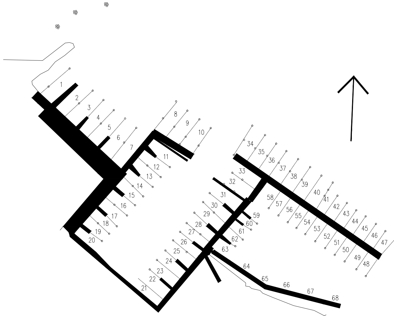
DOCK PLAN MIDDLESEX YACHT CLUB
